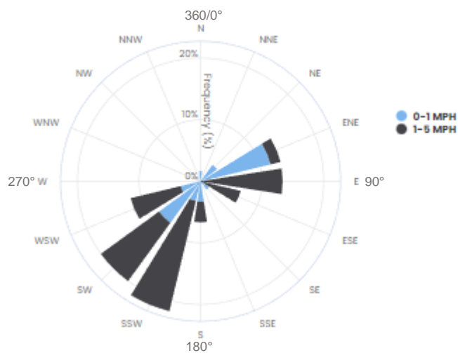
FIGURE 1-3 CM7 WIND ROSE | MAY 17, 2022, 9:30 P.M. - 10:30 P.M.
