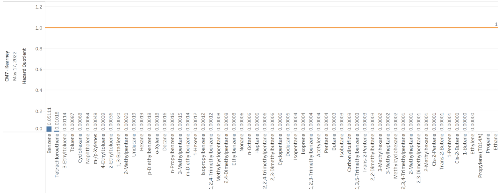
FIGURE 1-4 COMPOUND SPECIFIC HAZARD QUOTIENTS FOR VOCs DETECTED IN THE MAY 17, 2022 SENSOR-TRIGGERED EVENT SAMPLE AT CM7 KEARNEY MIDDLE SCHOOL LOCATION
