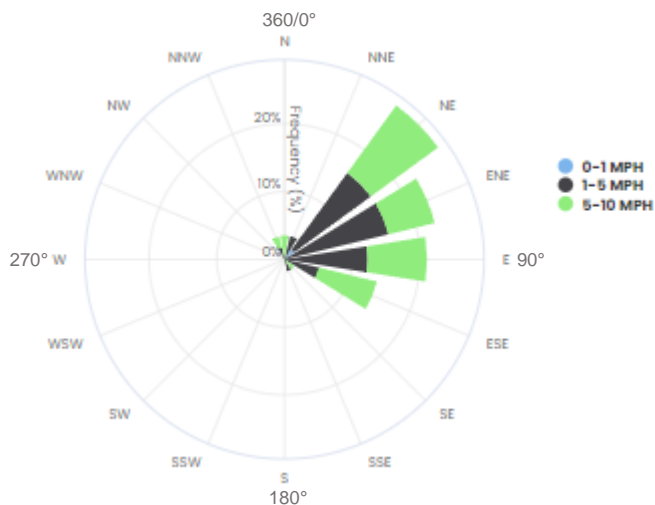
FIGURE 1-3 CM10 WIND ROSE | MAY 13, 2022, 2:30 P.M. - 3:30 P.M.
