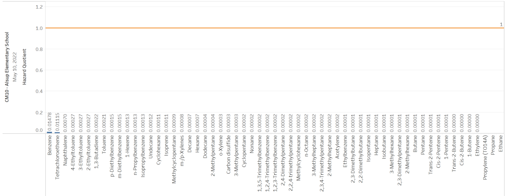
FIGURE 1-4 COMPOUND SPECIFIC HAZARD QUOTIENTS FOR VOCs DETECTED IN THE MAY 10, 2022 SENSOR-TRIGGERED EVENT SAMPLE AT CM10 ALSUP ELEMENTARY SCHOOL LOCATION
