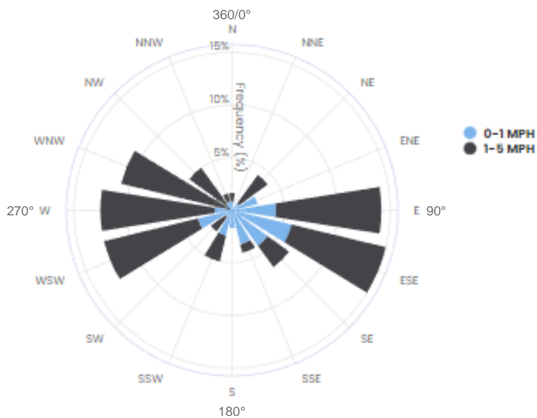
FIGURE 1-3 CM10 WIND ROSE | MAY 10, 2022, 9:30 P.M. - 11:30 P.M.
