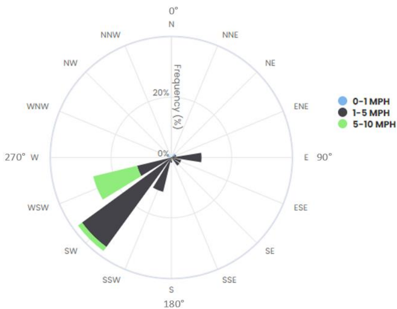
FIGURE 1-3 CM4 WIND ROSE | MARCH 1, 2022, 10:00 P.M. - 11:00 P.M.
