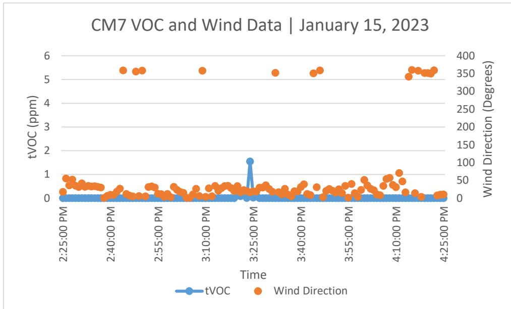
FIGURE 1-2 CM7 VOC AND WIND DIRECTION | JANUARY 15, 2023, 2:25 P.M. – 4:25 P.M.
