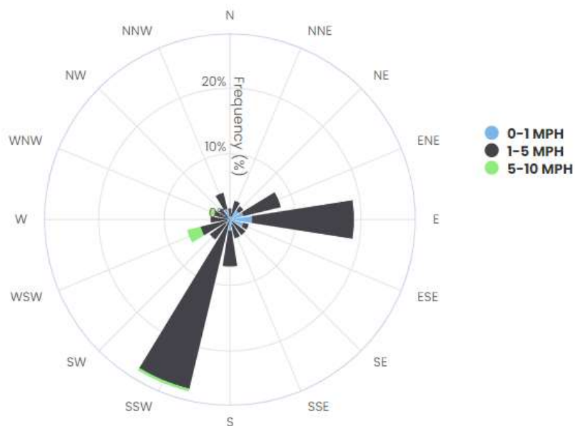
FIGURE 1-3 CM1 WIND ROSE | DECEMBER 24, 2021, 2:00 P.M. - 6:00 P.M.
