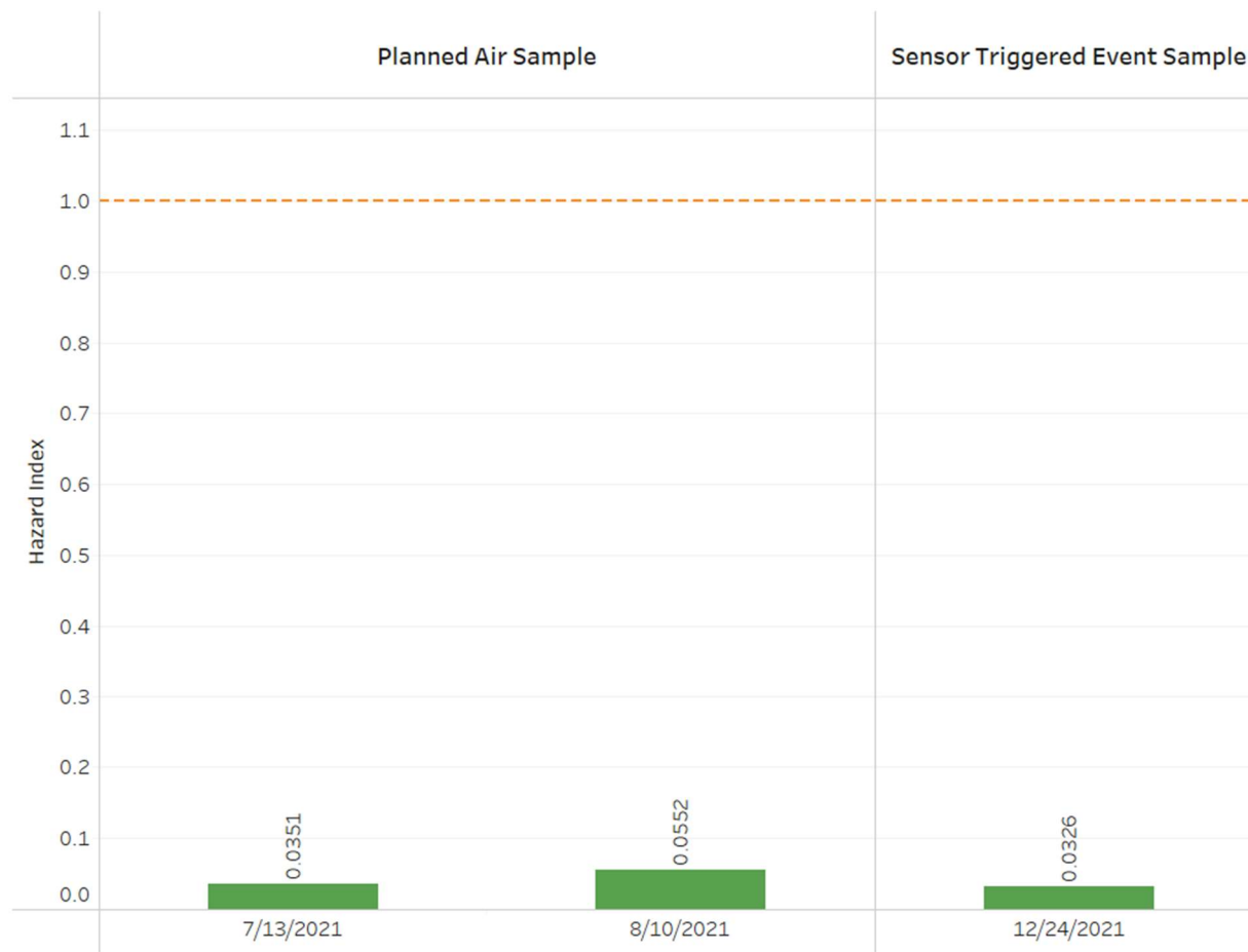
FIGURE 1-5 HAZARD INDICIES AT THE CCND CM1 - ROSE HILL ELEMENTARY SCHOOL LOCATION FOR PLANNED AND SENSOR TRIGGERED AIR SAMPLES
