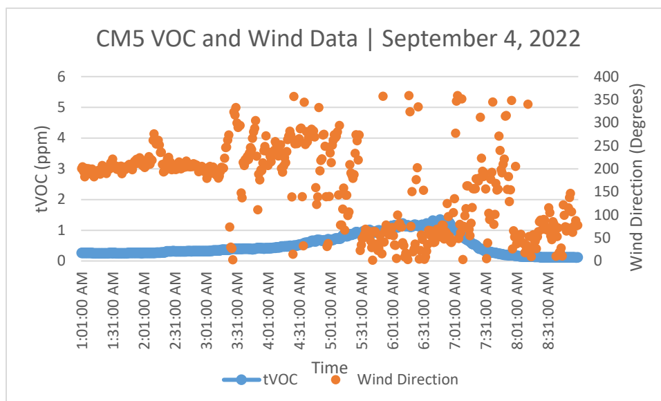
FIGURE 1-2 CM5 VOC AND WIND DIRECTION | SEPTEMBER 4, 2022, 1:00 A.M. – 9:00 A.M.
