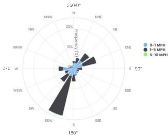
FIGURE 1-3 CM5 WIND ROSE | SEPTEMBER 4, 2022, 1:00 A.M. – 9:00 A.M.
