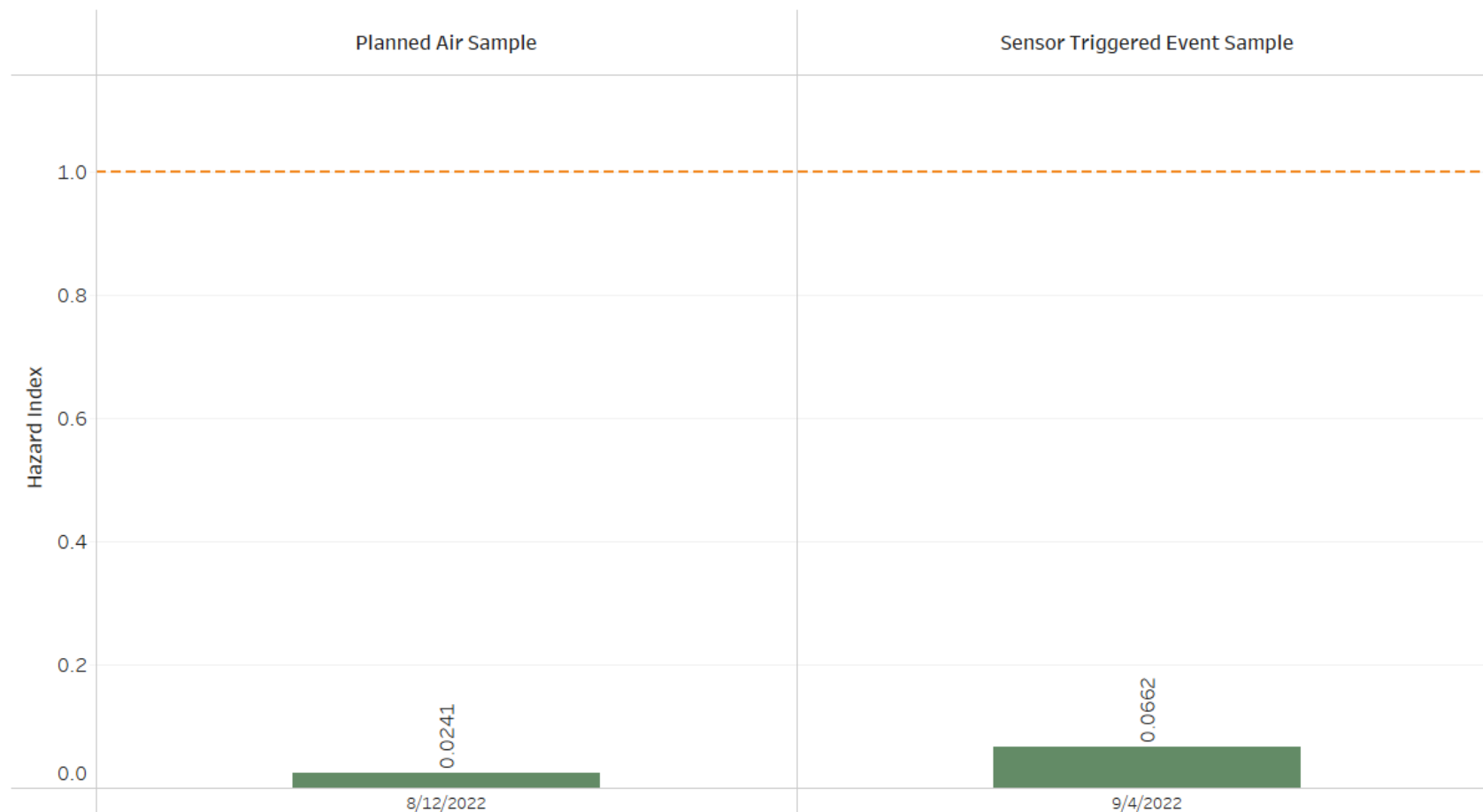
FIGURE 1-5 HAZARD INDICIES AT THE CCND CM5 - CENTRAL ELEMENTARY SCHOOL LOCATION FOR PLANNED AND SENSOR TRIGGERED AIR SAMPLES
