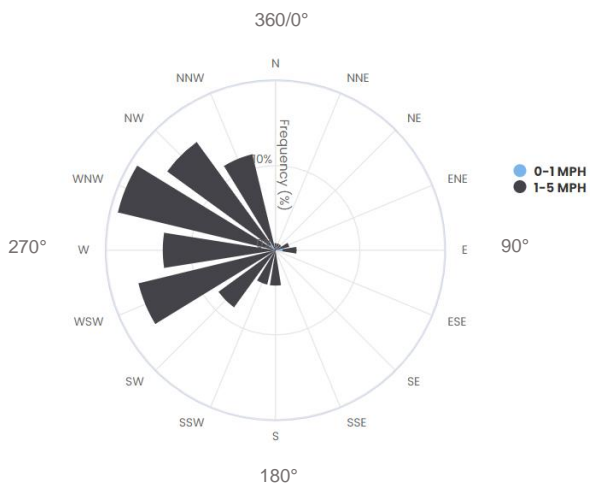
FIGURE 1-3 CM3 WIND ROSE | JULY 20, 2022, 2:30 A.M. – 4:30 A.M.
