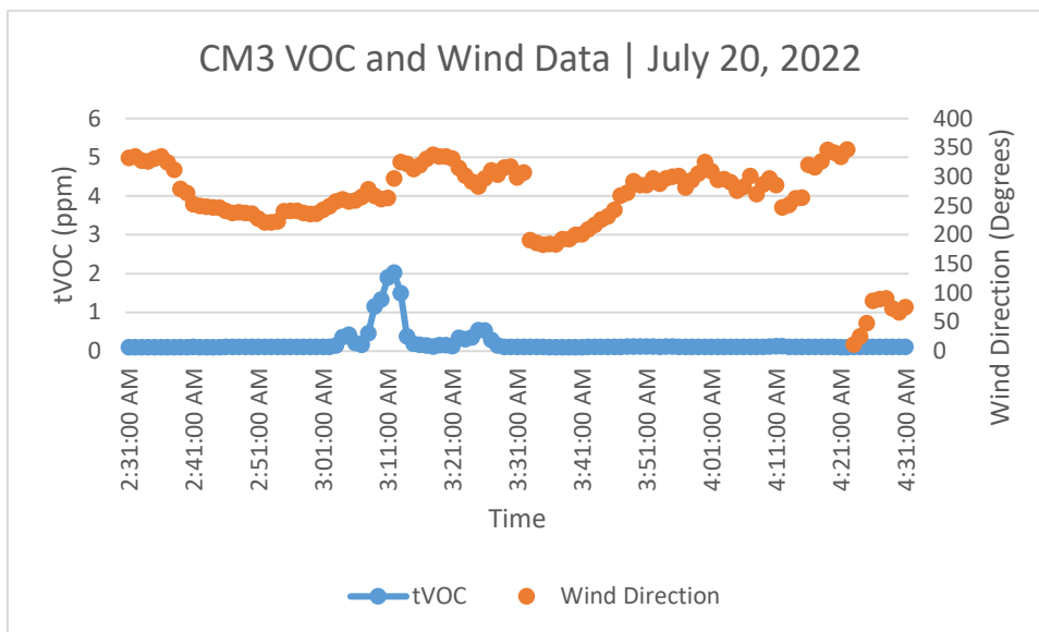
FIGURE 1-2 CM3 VOC AND WIND DIRECTION | JULY 20, 2022, 2:30 A.M. – 4:30 A.M.
