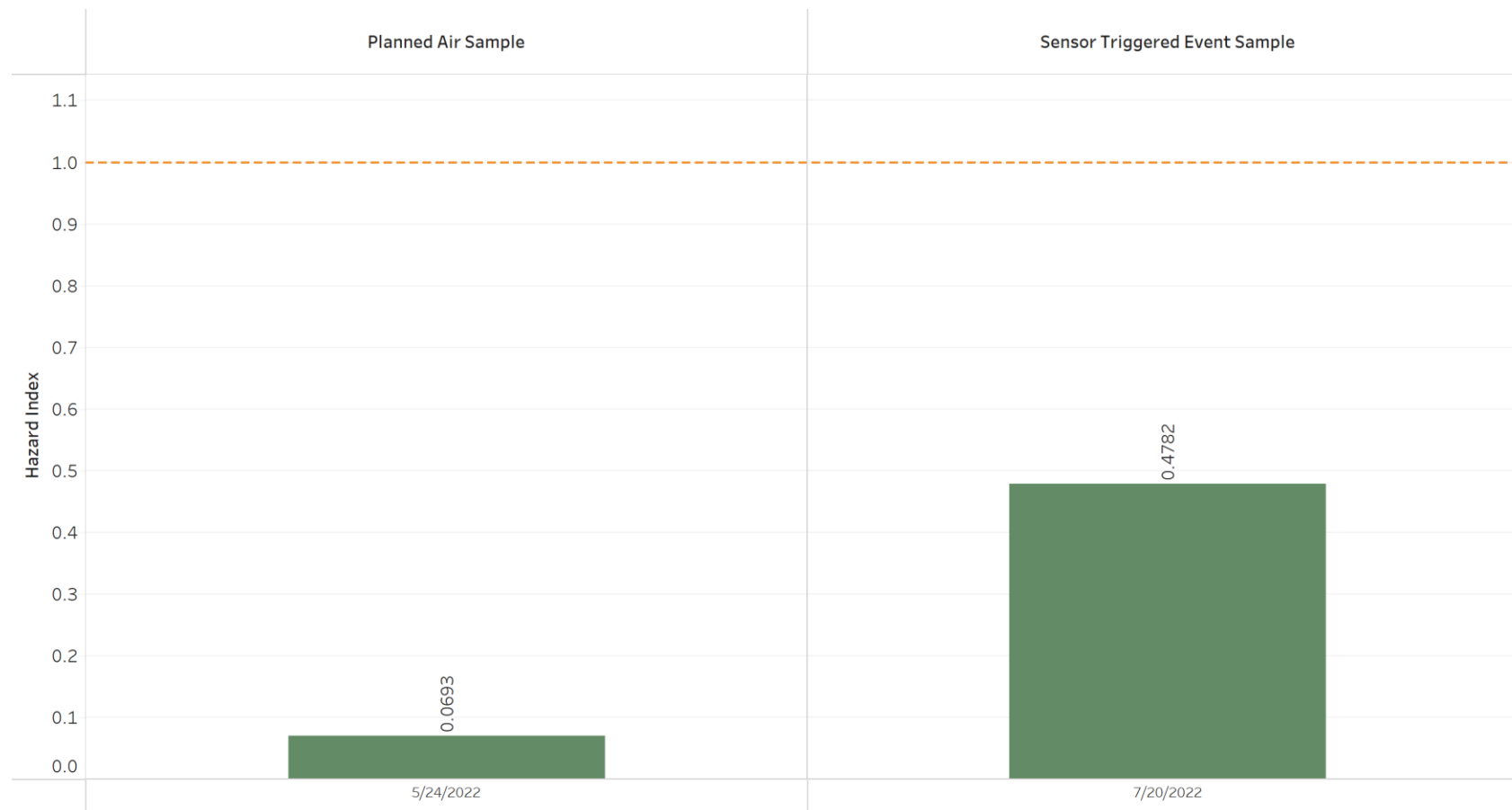
FIGURE 1-5 HAZARD INDICIES AT THE CCND CM3 - ADAMS HIGH SCHOOL LOCATION FOR PLANNED AND SENSOR TRIGGERED AIR SAMPLES
