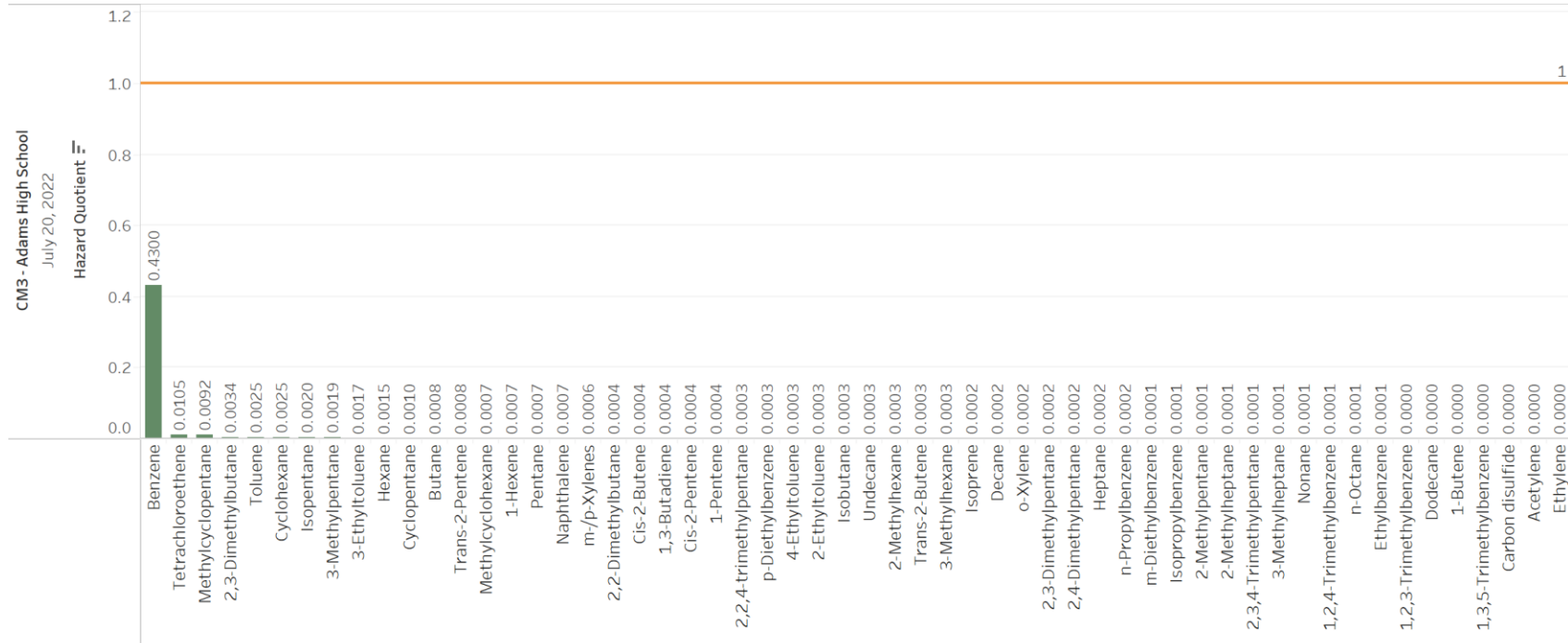
FIGURE 1-4 COMPOUND-SPECIFIC HAZARD QUOTIENTS FOR VOCs DETECTED IN THE JULY 20, 2022, SENSOR-TRIGGERED EVENT SAMPLE AT CM3 ADAMS HIGH SCHOOL LOCATION
