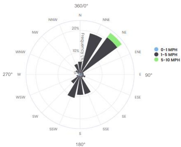
FIGURE 1-3 CM9 WIND ROSE | OCTOBER 17, 2022, 2:30 P.M. – 4:30 P.M.
