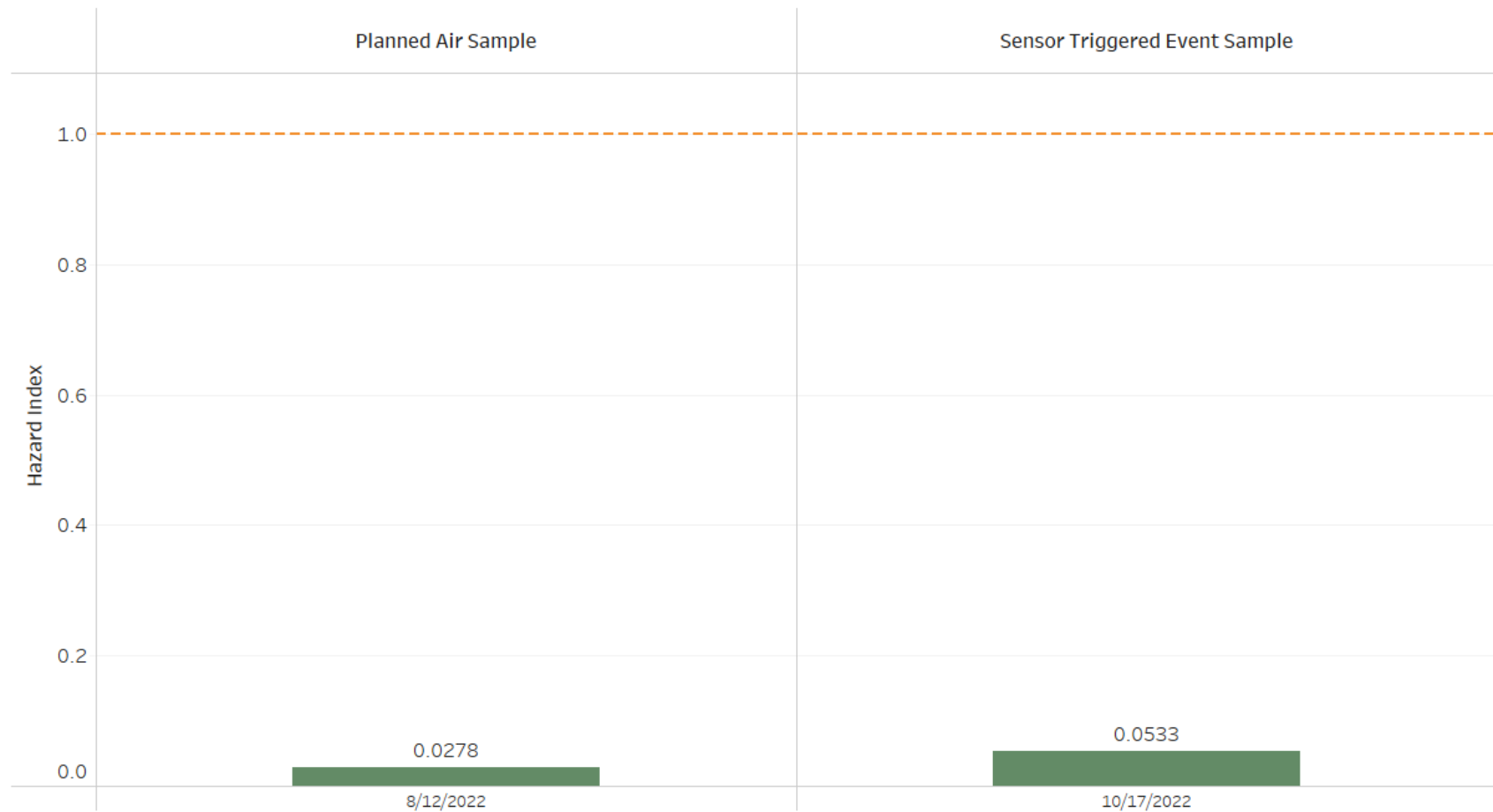
FIGURE 1-5 HAZARD INDICIES AT THE CCND CM9 – 48 TH AND RACE LOCATION FOR PLANNED AND SENSOR TRIGGERED AIR SAMPLES
