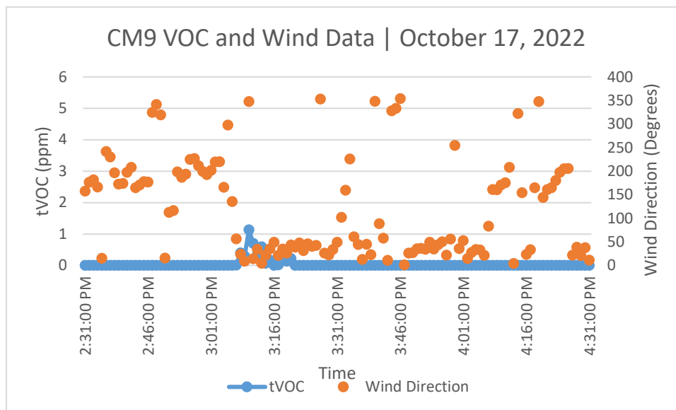
FIGURE 1-2 CM9 VOC AND WIND DIRECTION | OCTOBER 17, 2022, 2:30 P.M. – 4:30 P.M.
