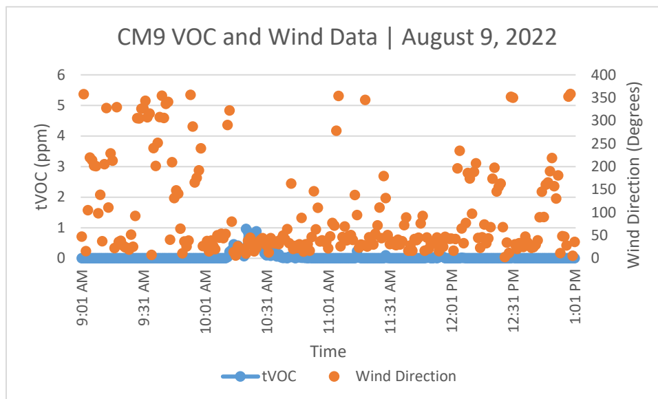
FIGURE 1-2 CM9 VOC AND WIND DIRECTION | AUGUST 9, 2022, 9:00 A.M. – 1:00 P.M.
