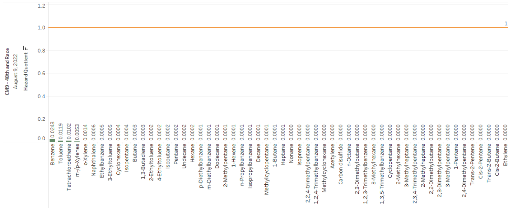
FIGURE 1-4 COMPOUND-SPECIFIC HAZARD QUOTIENTS FOR VOCs DETECTED IN THE AUGUST 9, 2022, SENSOR-TRIGGERED EVENT SAMPLE AT CM9 48TH AND RACE LOCATION
