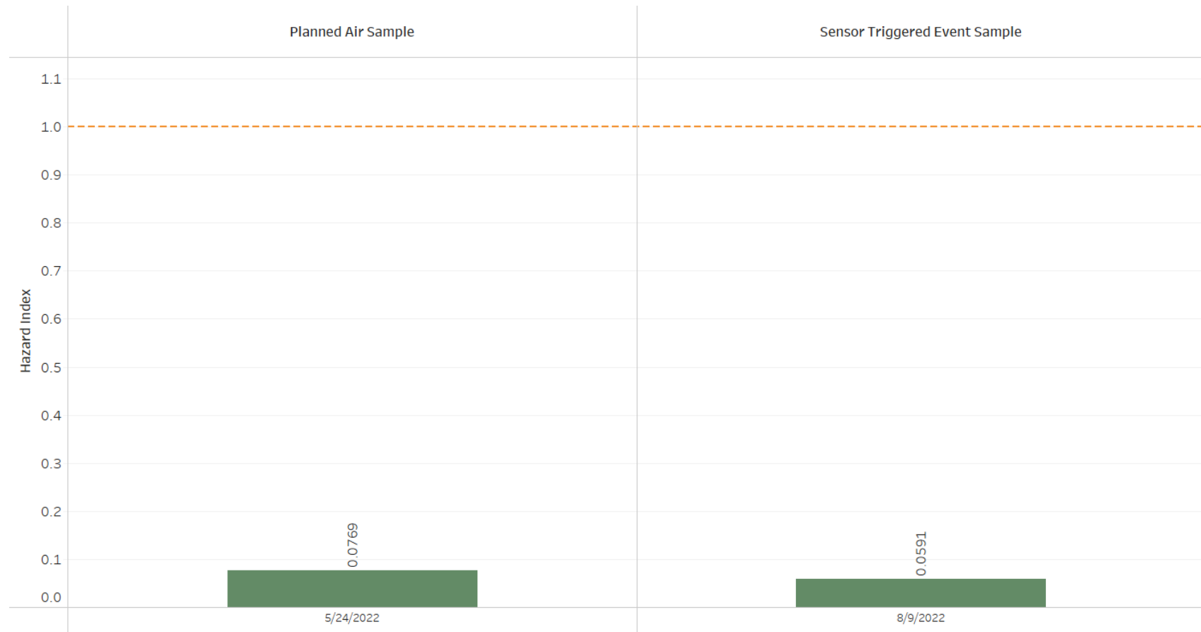
FIGURE 1-5 HAZARD INDICIES AT THE CCND CM9 - 48TH AND RACE LOCATION FOR PLANNED AND SENSOR TRIGGERED AIR SAMPLES
