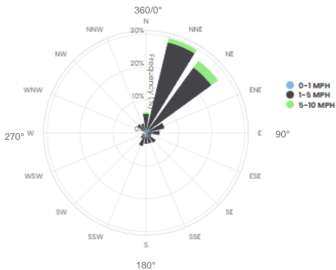
FIGURE 1-3 CM9 WIND ROSE | AUGUST 9, 2022, 9:00 A.M. – 1:00 P.M.
